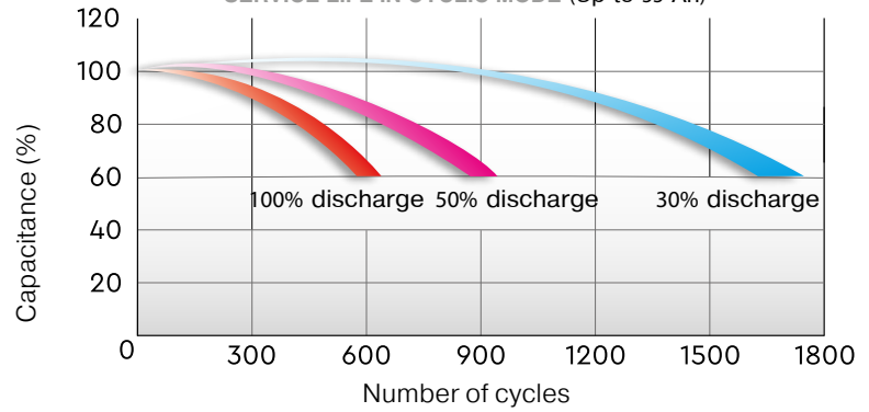
SERVICE LIFE IN CYCLIC MODE (Up to 55 Ah)
