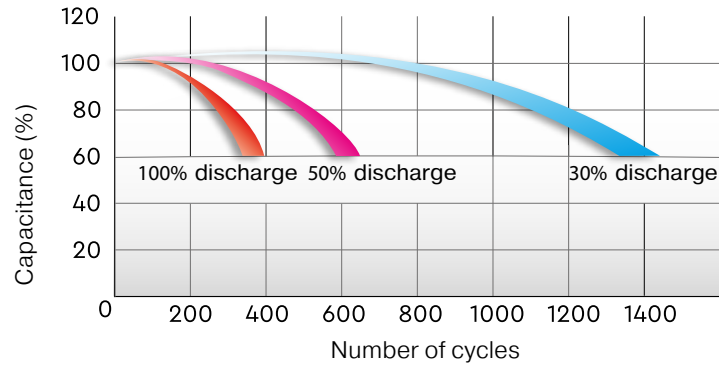
SERVICE LIFE IN CYCLIC MODE (Up to 60 Ah)
