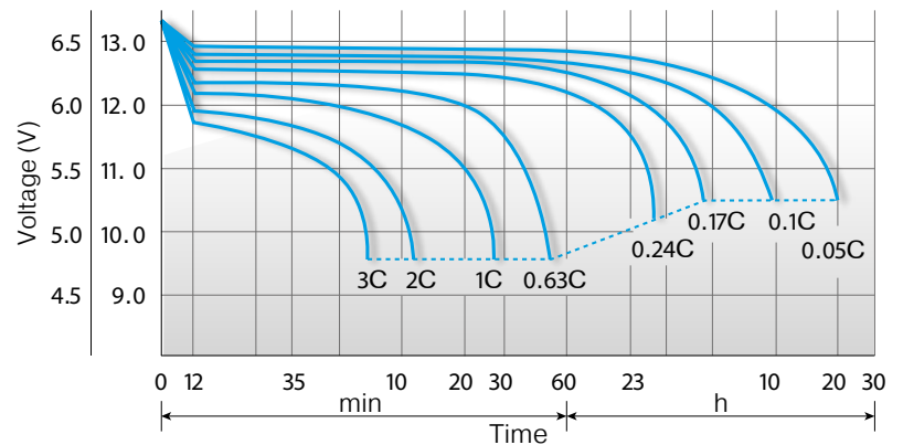
DISCHARGE CHARACTERISTICS
