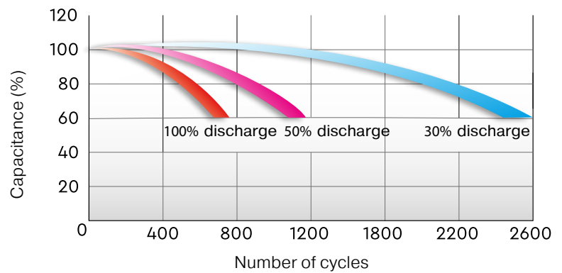
SERVICE LIFE IN CYCLIC MODE (Over 100 Ah)
