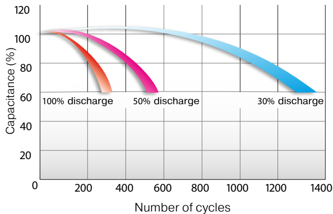
SERVICE LIFE IN CYCLIC MODE (Over 40 Ah)
