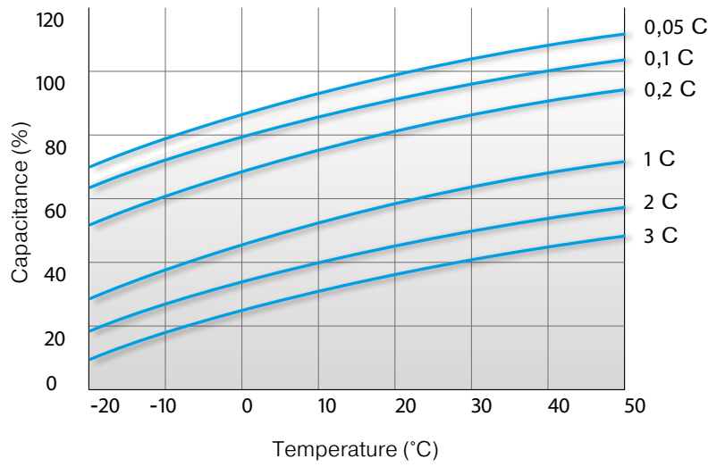
TEMPERATURE INFLUENCE ON THE CAPACITANCE
