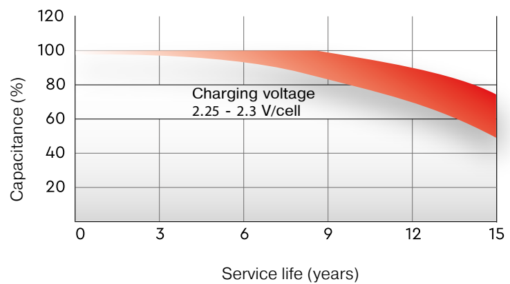
SERVICE LIFE IN BUFFER MODE
