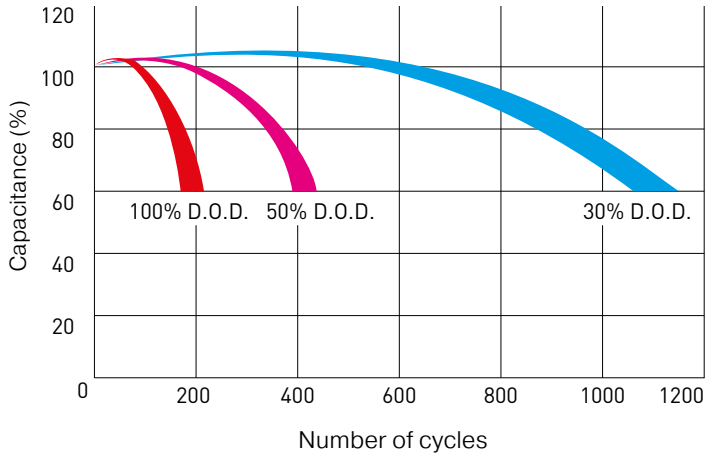
SERVICE LIFE IN CYCLIC MODE (Over 65 Ah)
