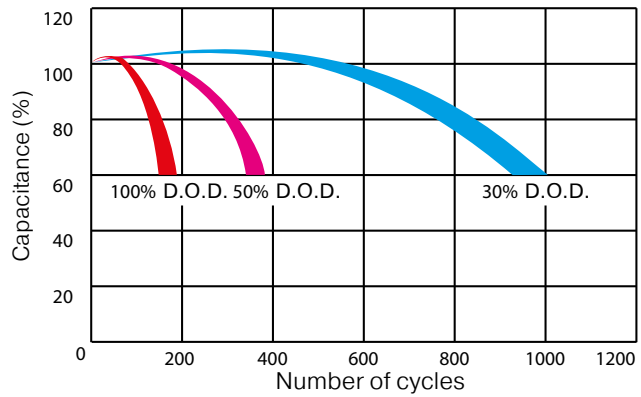
SERVICE LIFE IN BUFFER MODE (5 YEARS)
