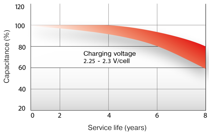
SERVICE LIFE IN BUFFER MODE (8 YEARS)
