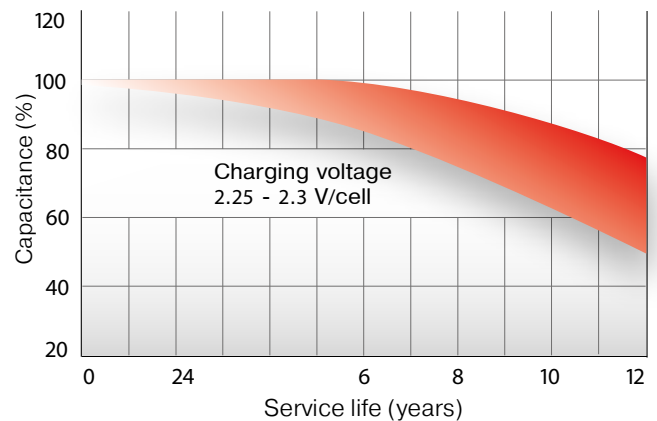
SERVICE LIFE IN BUFFER MODE (10 YEARS)
